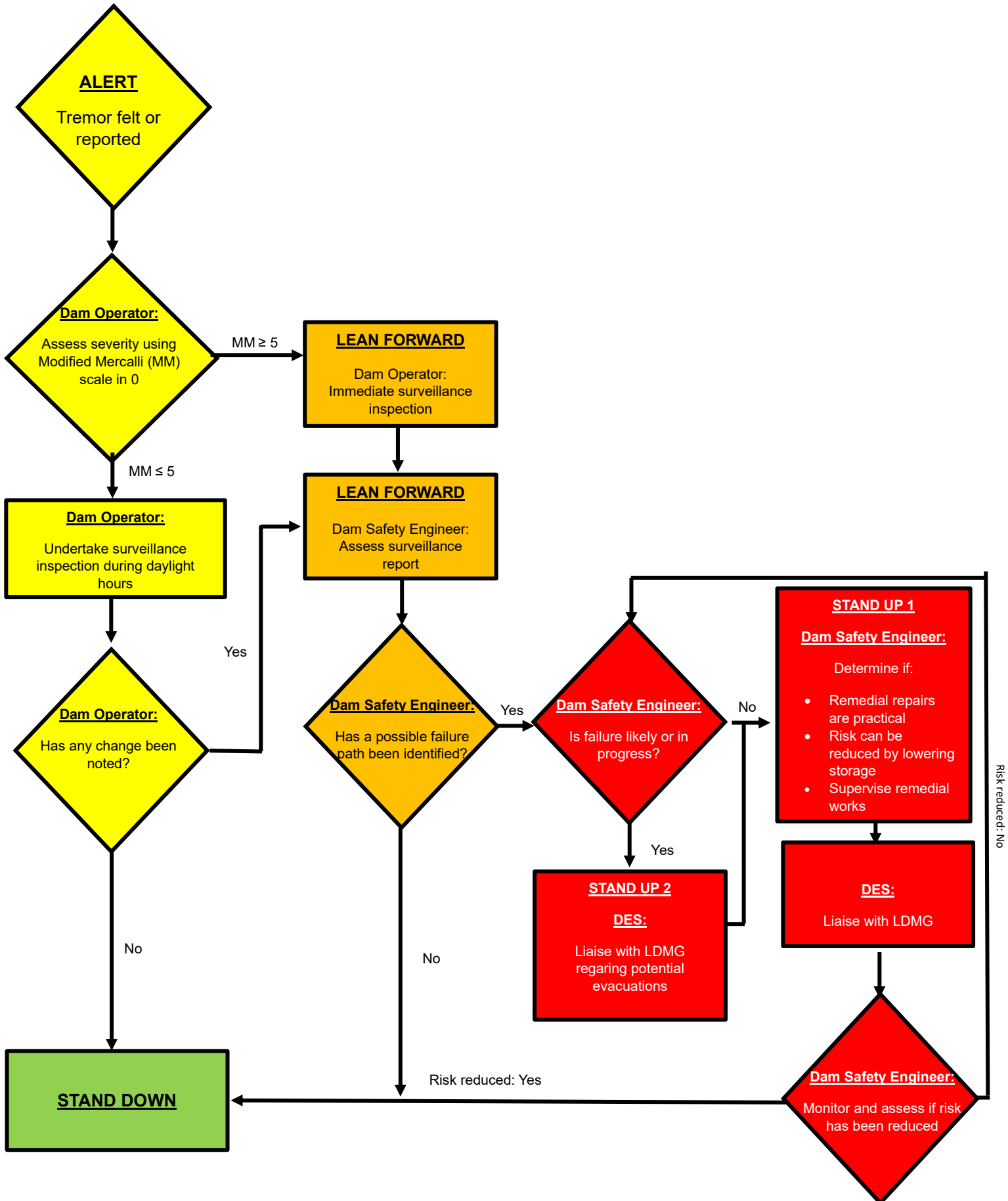
FIGURE 5-2 EARTHQUAKE FLOWCHART
